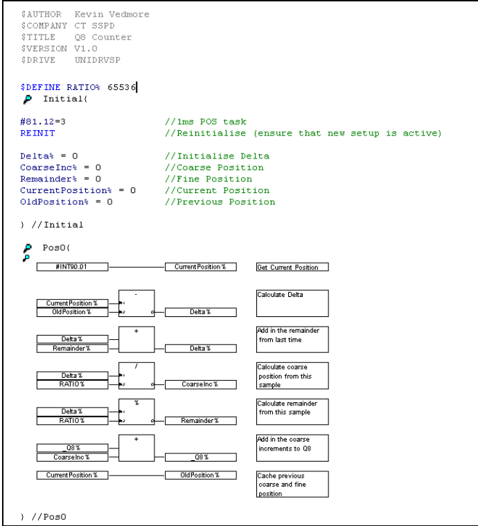
Figure 4-5 Example DPL Program
